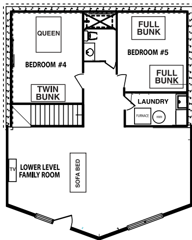
Lower Floor
